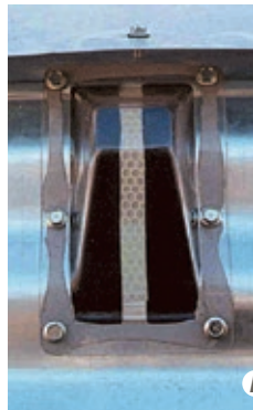
A B EasyFlow™ U-Trough unload system C Century Door with auger chute D 15" circular galvanized vent E Wider inspection hatch F Grain Gauge™ G Ultra-flat 4" wide corrugation pattern H Pass through rail (optional)
